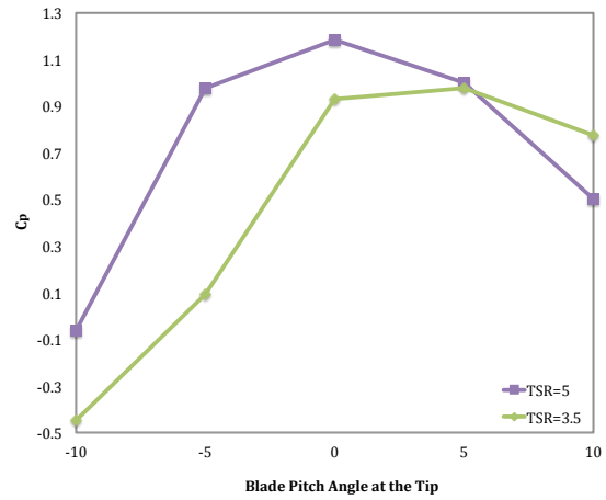
FIGURE 13. POWER COEFFICIENT AT TSR=5 AND 3.5 VERSUS PITCH ANGLE FOR 16 M WIDE CHANNEL.
