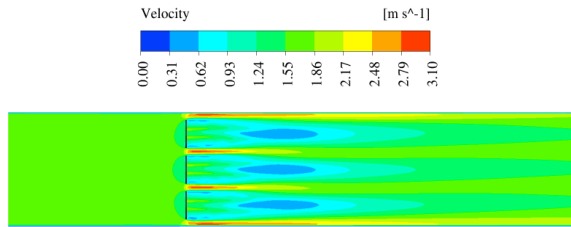
FIGURE 11. TOP VIEW VELOCITY CONTOUR PLOT OF THE OPTIMIZED TURBINE DESIGN (TSR=5 AND \theta_{p,0} = 0 ) AT THE PLANE PASSING THROUGH THE CENTER OF TURBINE.
