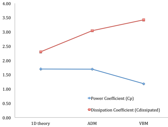
FIGURE 15. COMPARISON BETWEEN ONE-DIMENSIONAL THEORY, ADM AND VBM FOR POWER COEFFICIENT AND DISSIPATION COEFFICIENT AT TSR=5 AND \theta_{p,0} = 0 .
