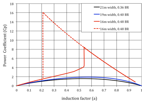
FIGURE 6. EFFECT OF CHANNEL CONSTRICTION ON POWER PRODUCTION
