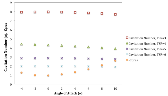
FIGURE 4. CAVITATION NUMBER AND MINIMUM NEGATIVE PRESSURE COEFFICIENT VERSUS ANGLE OF ATTACK (AT \theta_{p,0} = 0 ).
