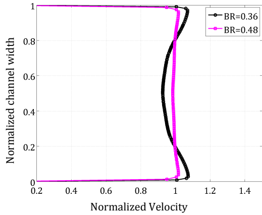
FIGURE 8. NORMALIZED VELOCITY VERSUS THE NORMALIZED CHANNEL WIDTH 1D UPSTREAM OF THE TURBINES.
