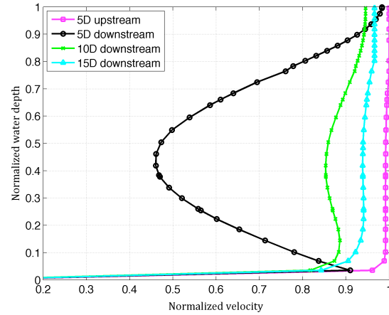
a) 16m wide channel
