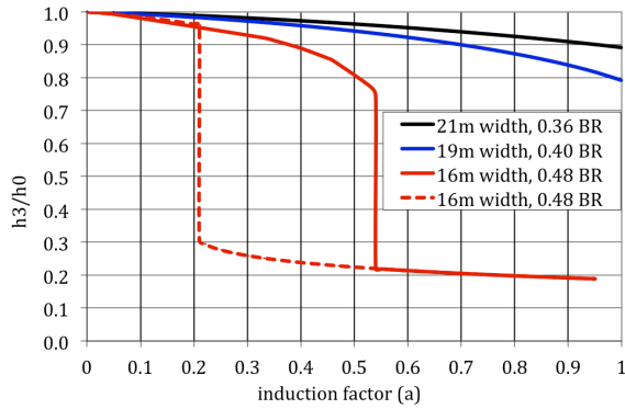
FIGURE 5. EFFECT OF CHANNEL CONSTRICTION ON SURFACE DROP AT THE END OF THE EXPANSION REGION.
