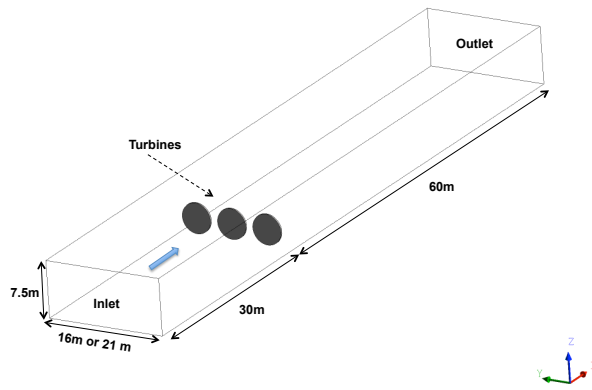
FIGURE 2. GEOMETRY OF THE COMPUTATIONAL DOMAIN
