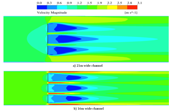
FIGURE 7. TOP VIEW OF VELOCITY MAGNITUDE PLOTS ON A PLANE PARALLEL TO THE CHANNEL BED PASSING THROUGH THE CENTER OF DISCS. A) 21M WIDE CHANNEL, BR=0.36, FR=0.18 B) 16M WIDE CHANNEL (SUBCRITICAL), BR=0.48, FR=0.24
