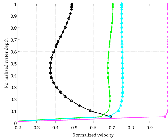
b) 21m wide channel
