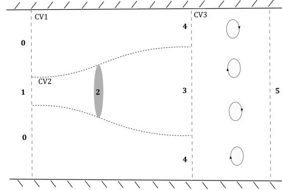
FIGURE 1. TOP VIEW OF ONE-DIMENSIONAL ACTUATOR DISC MODEL IN OPEN CHANNEL FLOW.
