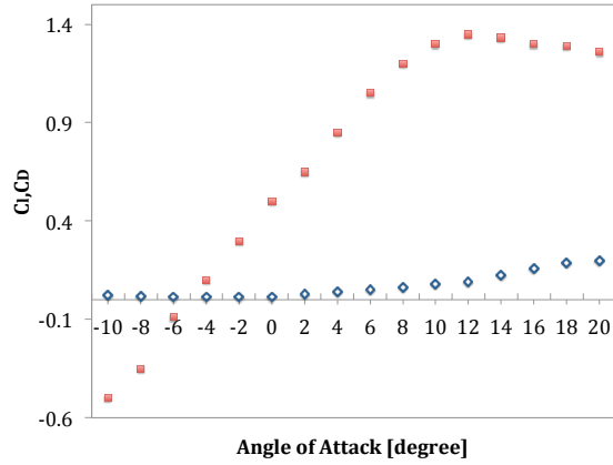
FIGURE 3. LIFT COEFFICIENT VERSUS ANGLE OF ATTACK FOR NACA 63-815 AIRFOIL [16].
